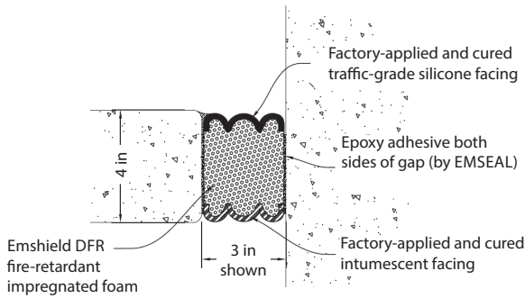
Deck to Wall
