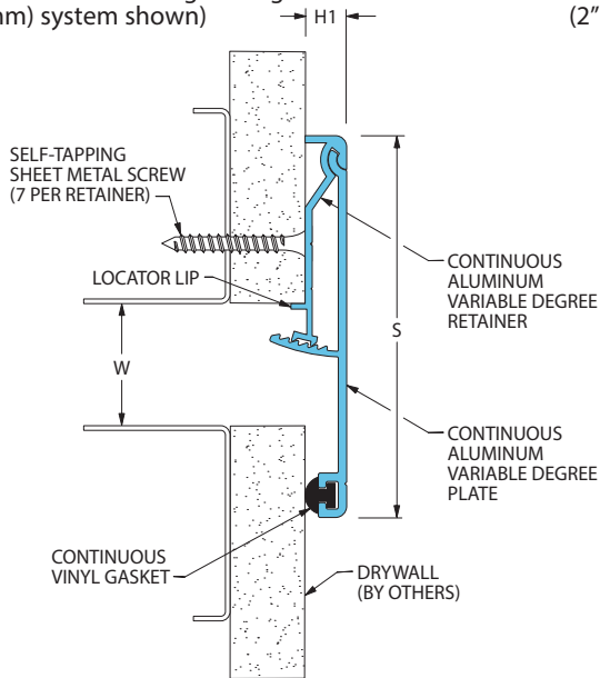
811-A07 Wall/Wall Ceiling/Ceiling (1" (25mm) system shown)
