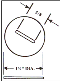
PRONG WASHER (R175P)
