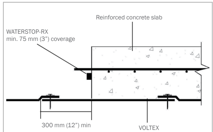
Figure 1.3 – Extend VOLTEX a minimum 300 mm (12") beyond slab edge. Install WATERSTOP-RX in joint
