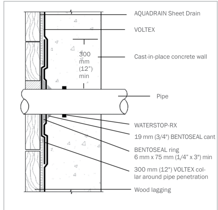
Figure 2.1 - WALL PENETRATION - Cut and secure VOLTEX tightly around penetrations and then apply BENTOSEAL 19 mm (3/4") ring around penetration and extend over membrane a minimum 75 mm (3") radius at minimum 6 mm (1/4") thickness
