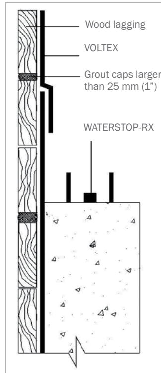
Figure 2.7 - VOLTEX installed directly to wood lagging with gaps filled. (Cast-in-place concrete wall)
