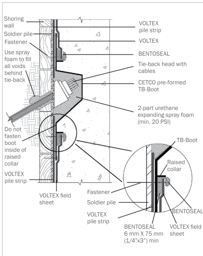
Figure 2.3a: TIE-BACK DETAIL – Install TB-Boot centered over tie-back then install VOLTEX with BENTOSEAL detailing. Do not fasten boot inside of raised collar around center formed area
