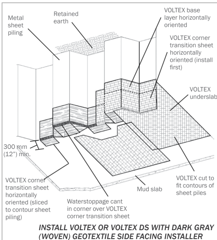
Figure 1.26 – Metal sheet piling to slab transition detail
