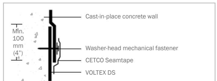
Figure 3.5 – Minimum VOLTEX overlap detail; tape VOLTEX DS seams
