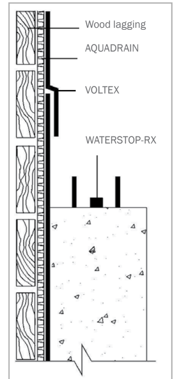
Figure 2.8 - AQUADRAIN used to cover gaps in lagging less than 63 mm (2.5"). (Cast-in-place concrete wall)
