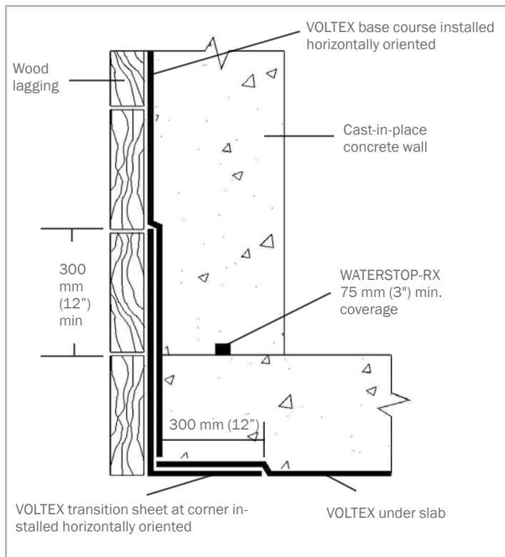
Figure 1.23 – SLAB-TO-WALL TRANSITION – VOLTEX corner transition sheet should extend past the height of the top of the finished slab level a minimum 300 mm (12") and extend under the slab 300 mm (12")
