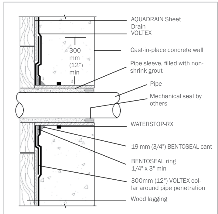
Figure 2.2 - SLEEVED WALL PENETRATION - Cut and secure VOLTEX tightly around penetrations and then apply BENTOSEAL 19 mm (3/4") ring around penetration and extend over membrane a min. 75 mm (3")
