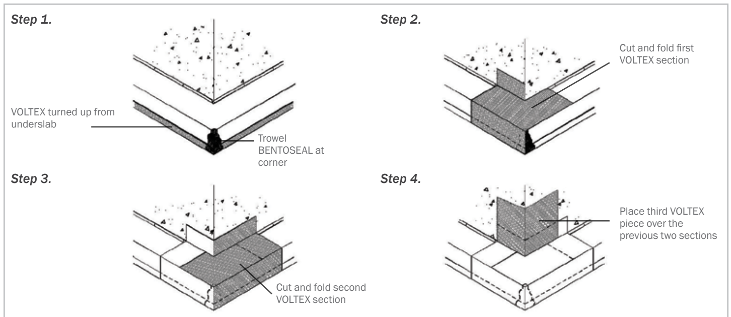
Figure 3.6 – Step by step detail of outside wall base corner installation (hydrostatic condition)
