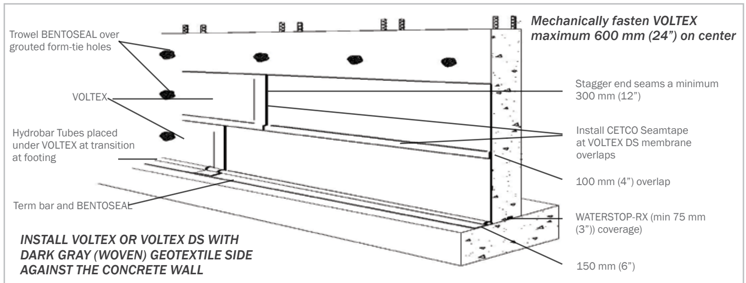
Figure 3.4 – VOLTEX installed on cast-in-place backfilled wall, overlap edges 100 mm (4") and stagger vertical end laps
