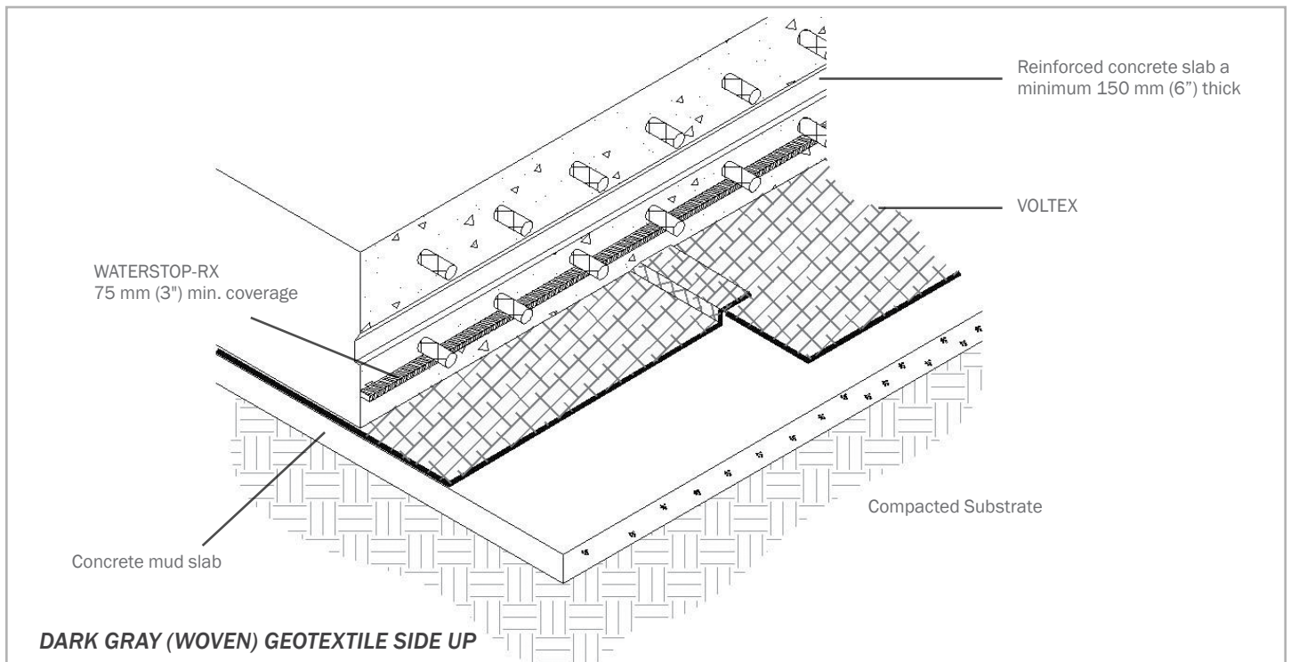
Figure 1.5 – VOLTEX installed over a mud slab requires a minimum 150 mm (6") thick reinforced slab
