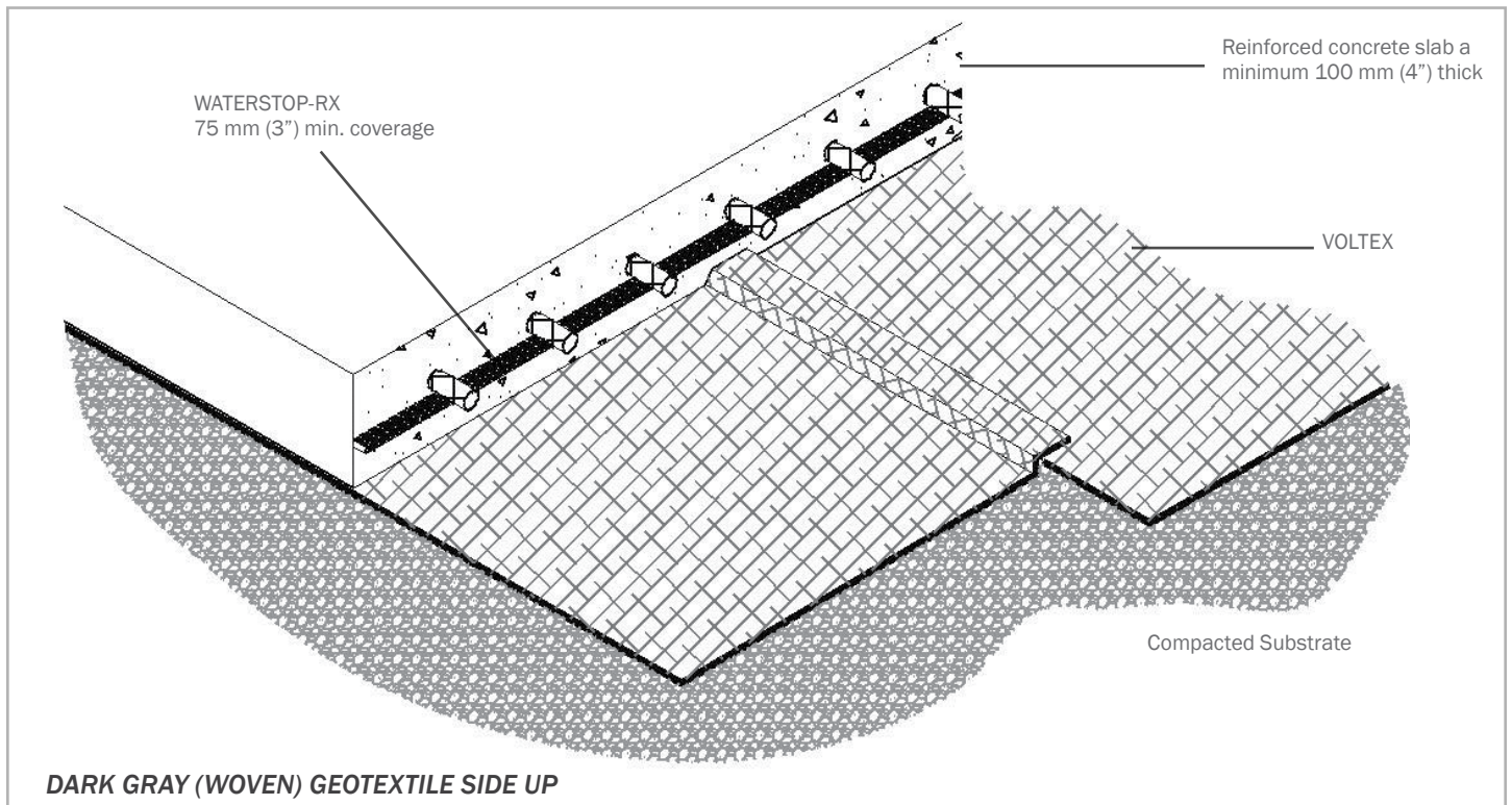
Figure 1.4 – VOLTEX installed directly over compacted earth/gravel substrate requires a minimum 100 mm (4") slab
