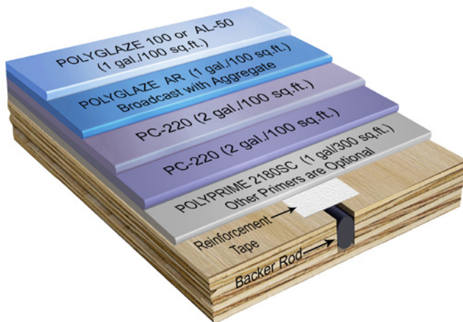
Plywood/Concrete Substrate
